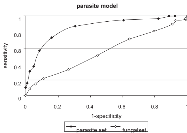
Fig. (1). ROC curve of the parasite model.
